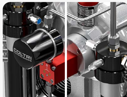
Safety valves after each stage of compression
